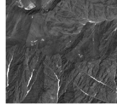
Green
