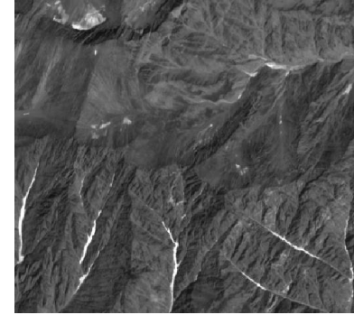
Red
