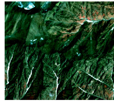
FCC
