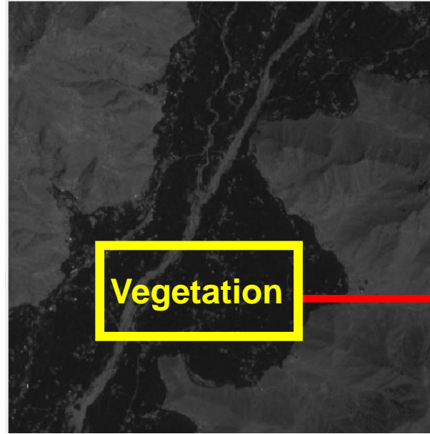
Red band
