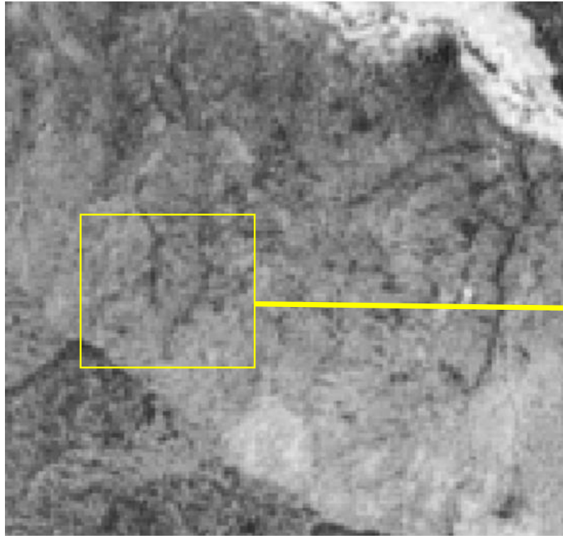
Normalized difference vegetation indices (NDVI)
