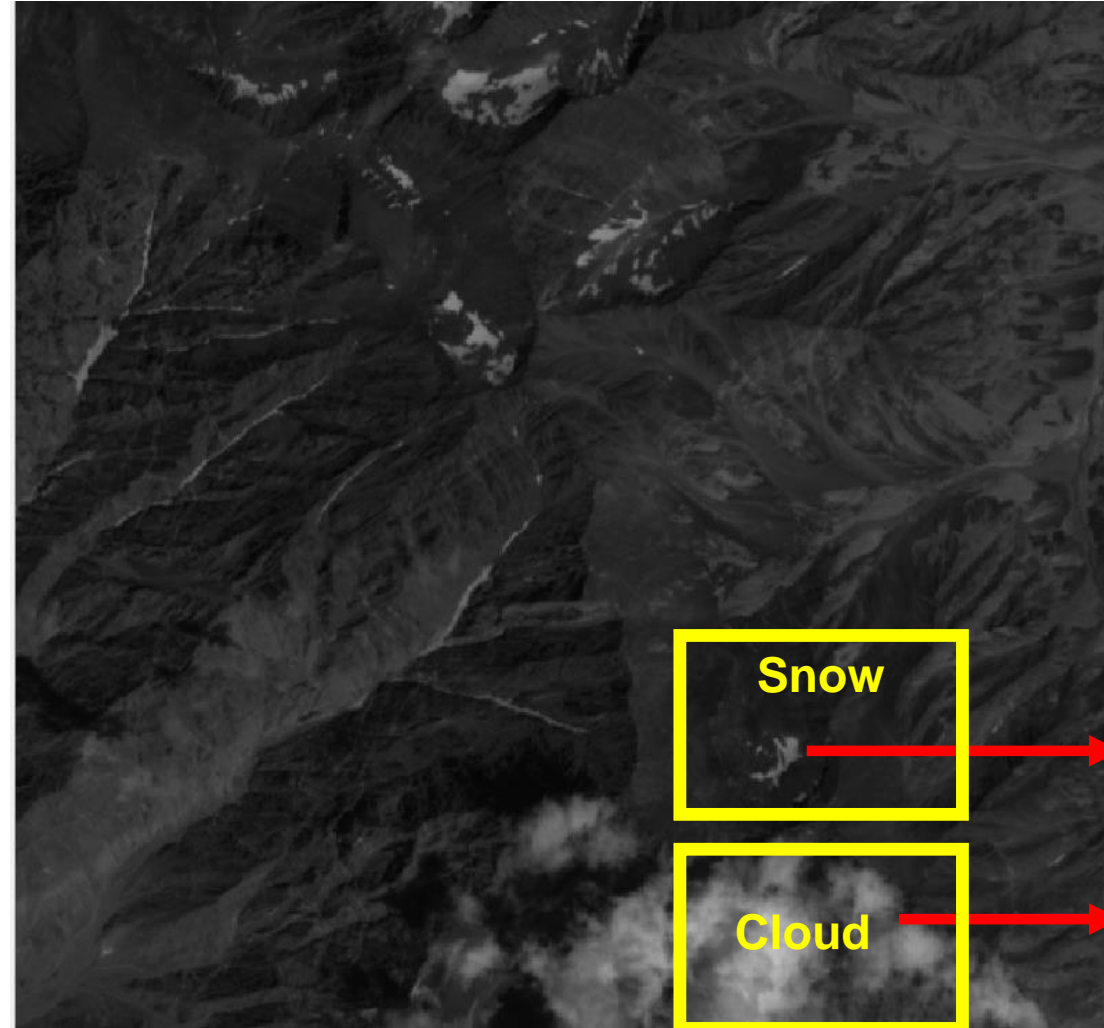
NIR band
