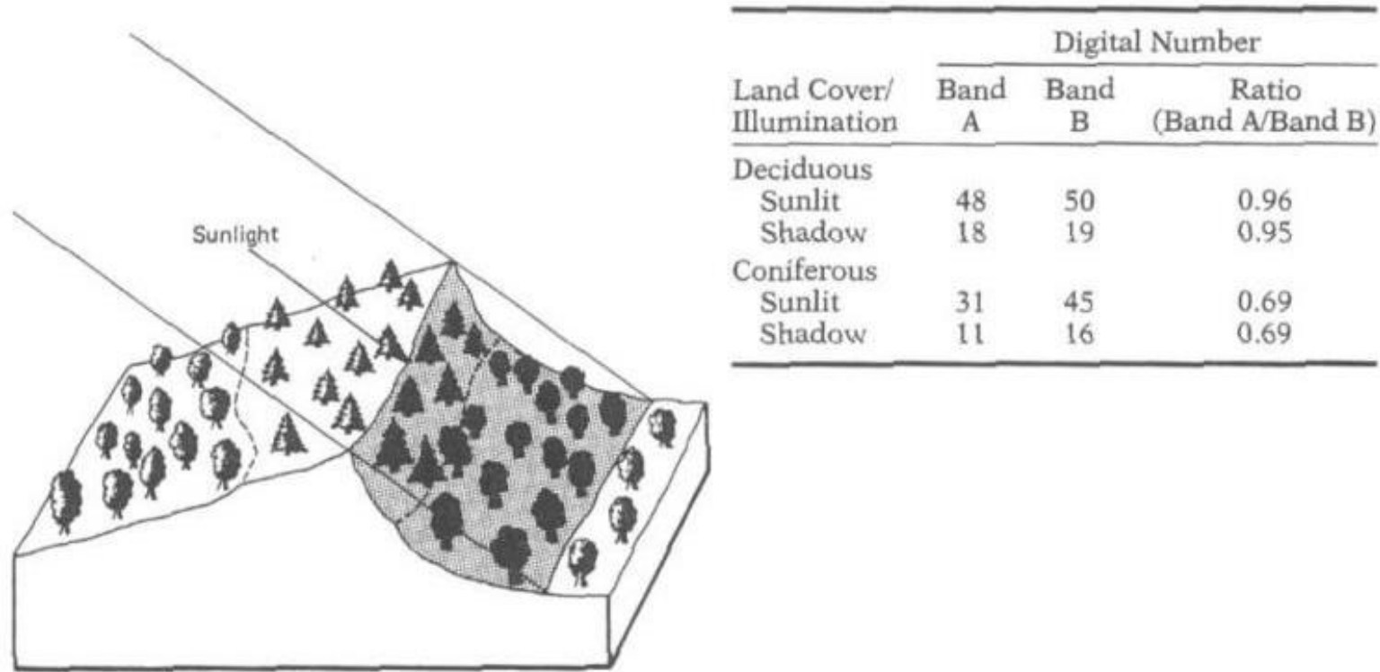
Figure 7.25 Reduction of scene illumination effects through spectral ratioing. (Adapted from Sabins, 1997.)
