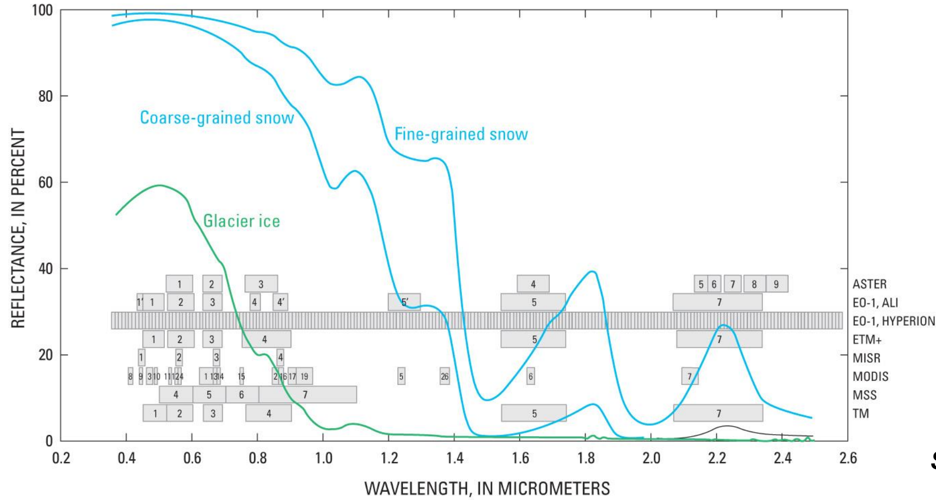
Spectral reflectance curves of bare glacier ice, coarse-grained snow, and fine-grained snow. Spectral bands of selected sensor on Earth-orbiting satellites are shown in gray. The numbers in the gray boxes refer to the associated band numbers of each sensor
